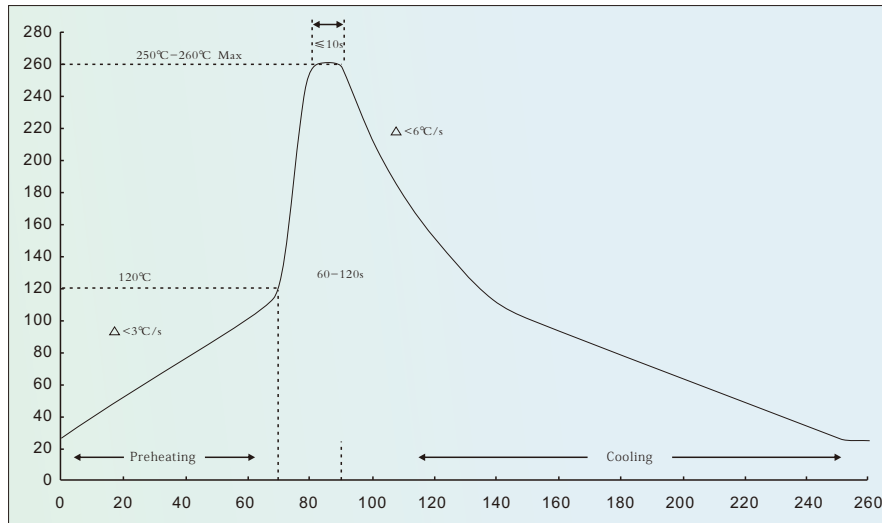
图二：波峰焊接温度曲线 Fig2:wave Soldering Profile
