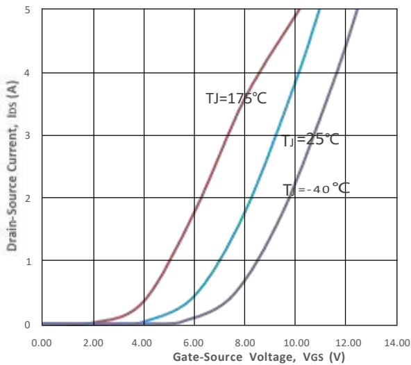
Fig5. Transfer Characteristic
