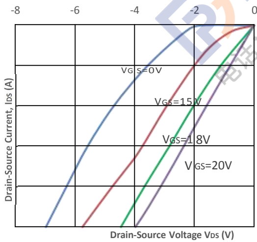
Fig9. 3rd Quadrant Characteristic at 25 ^{\circ} C
