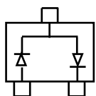
BAS70-04 Marking: 74
