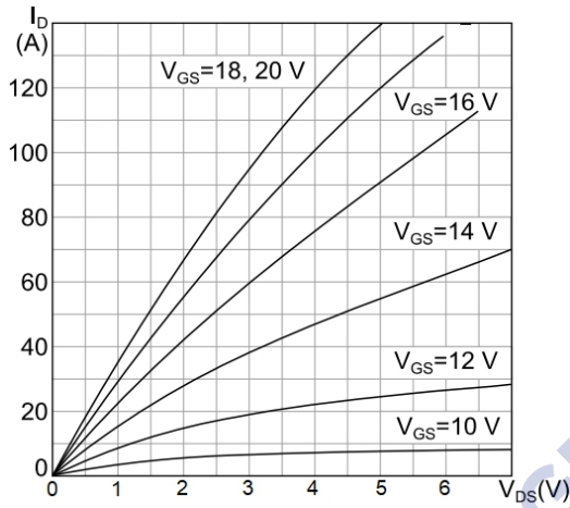
Figure 1: Output characteristics ( T_J = 25\text{ °C} )
