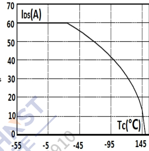
Figure 14: Continuous I_{DS} VS T_c
