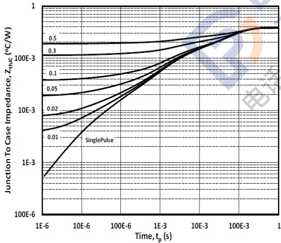
Figure 15: Thermal impedance
