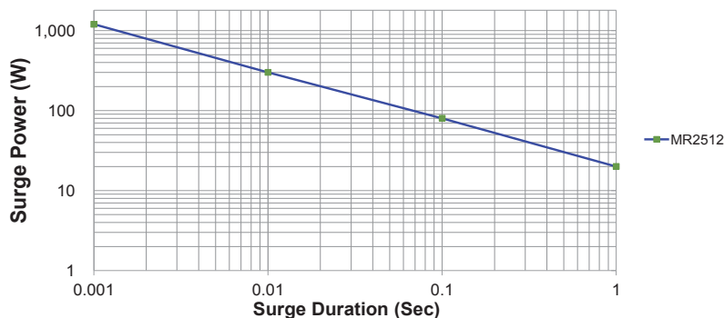
MR2512**G P-T Single Surge Curve
