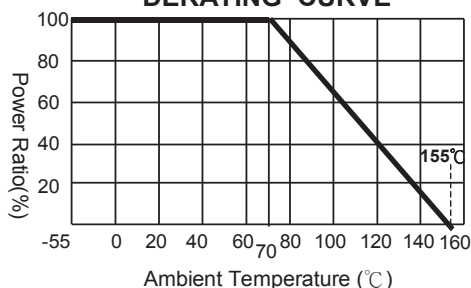
DERATING CURVE
