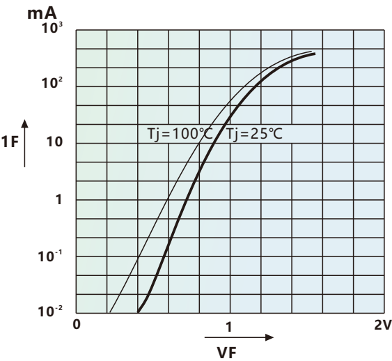
正向特性Figner 1.Forward characteristic
