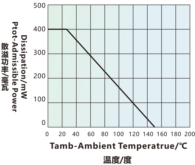
功率衰减Ffigure 2.Power De-rating
