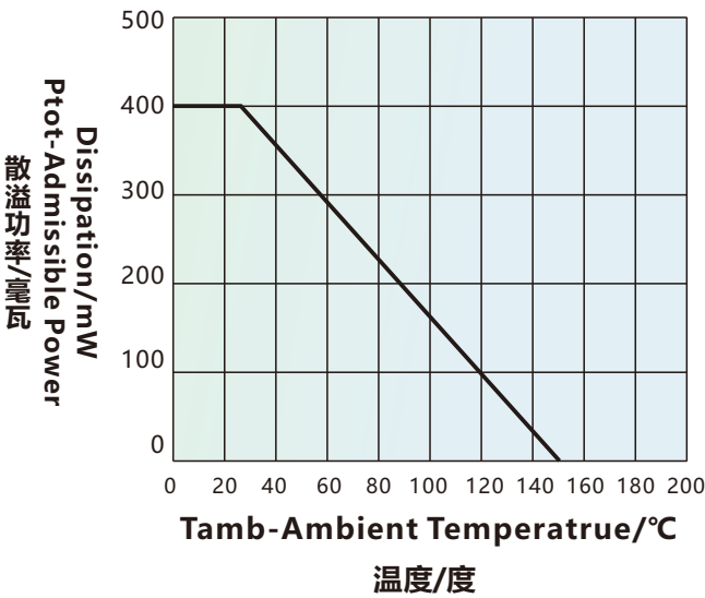
功率衰减Figure 2.Power De-rating
