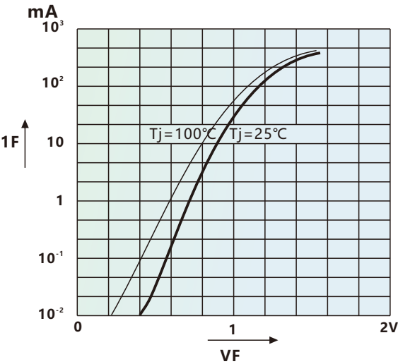
正向特性Figure 1.Forward characteristic
