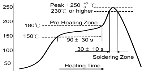
Reflow Soldering
