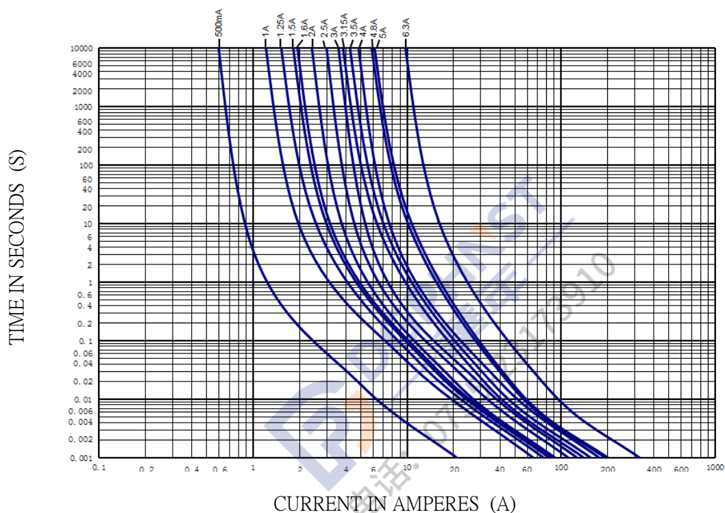
8-3 I-t 图/CHARACTERISTICS DIAGRAM(I-t)
