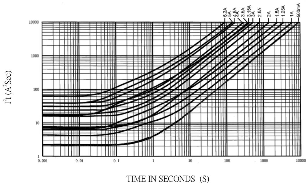
8-4 I^2t -t 图/CHARACTERISTICS DIAGRAM( I^2t -t)
